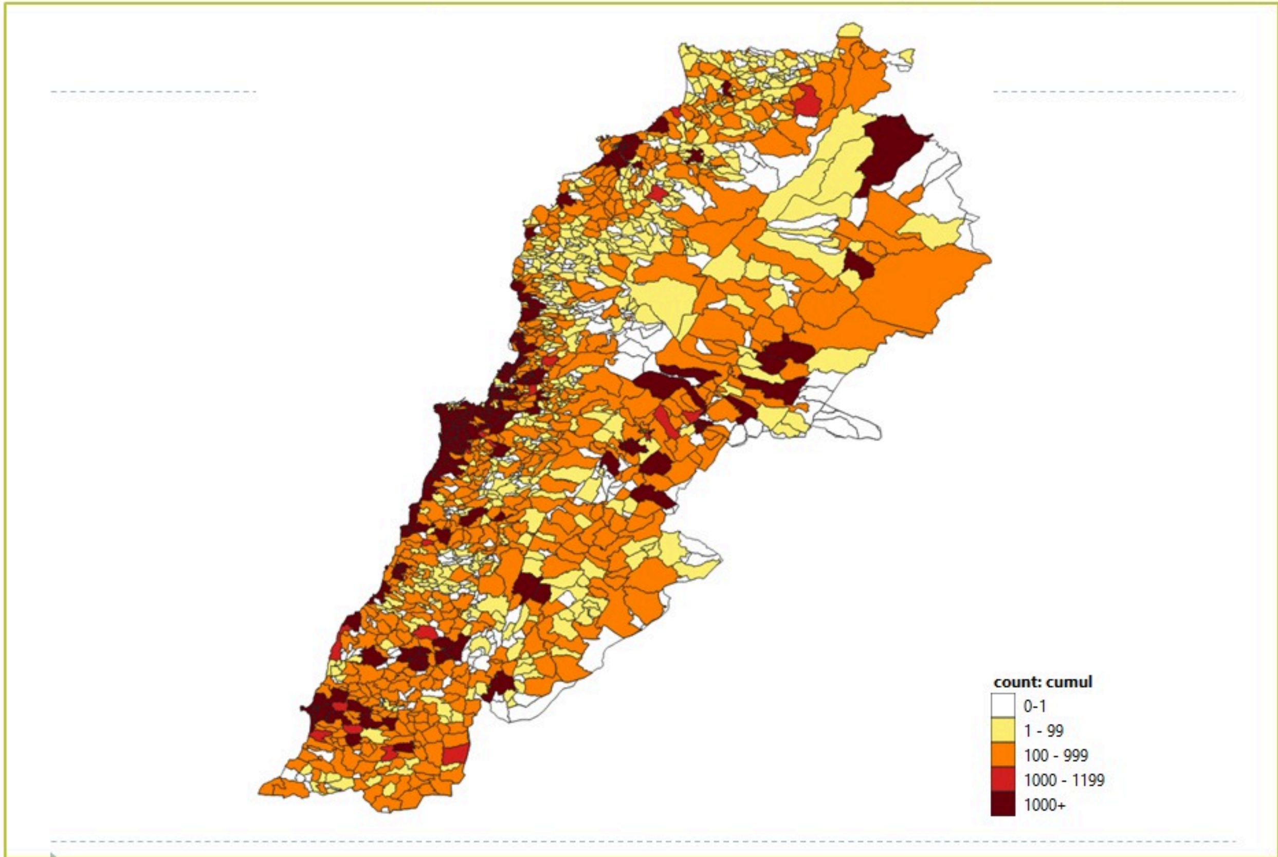
Map of distribution of cumulative number of cases by locality – 16 February 2022
