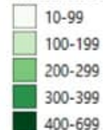
incidence rate: past 14 days per 100000
