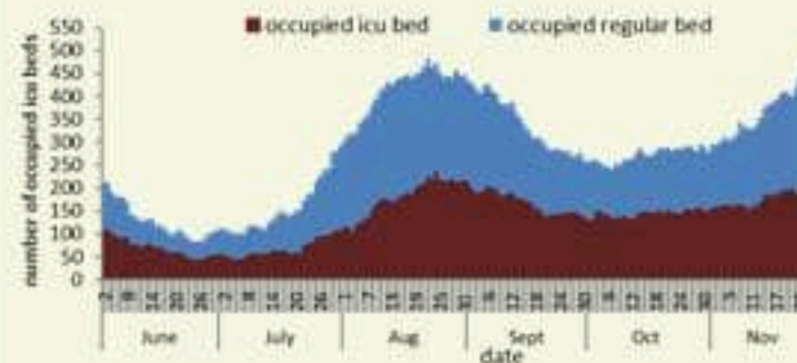
COVID19 hospital bed occupancy per day
